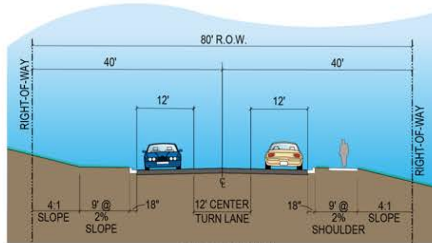
STREET SECTION
