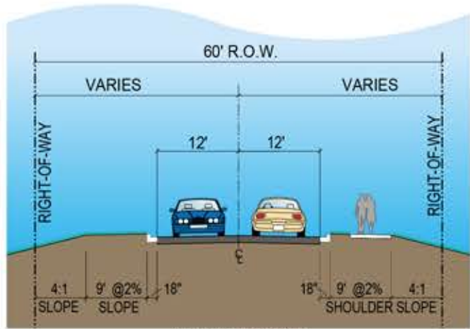
STREET SECTION
