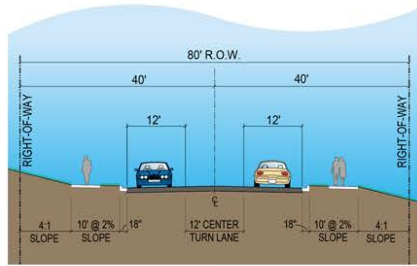
STREET SECTION
