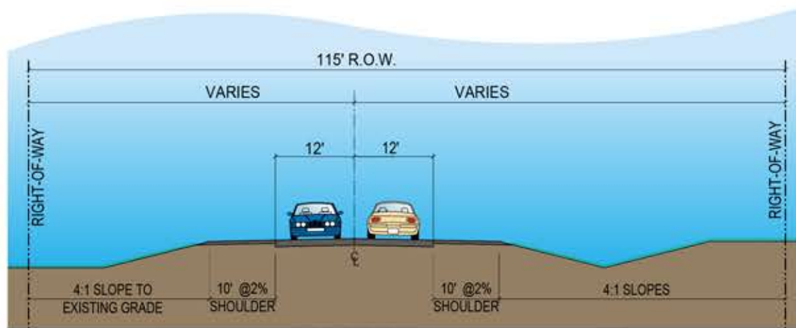
STREET SECTION
